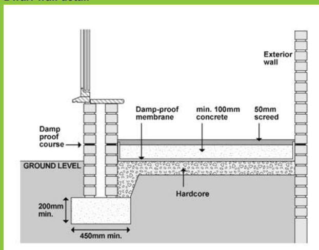
Dwarf wall detail
