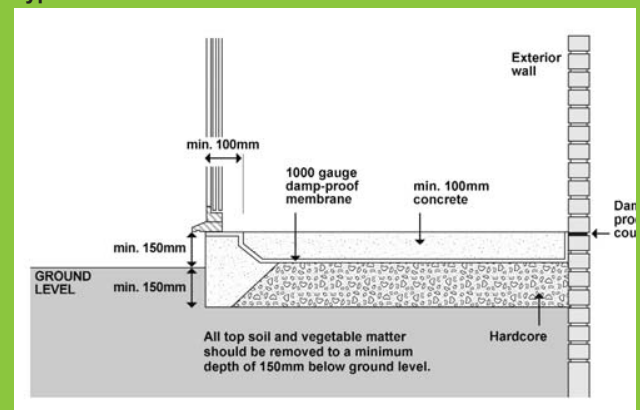
Typical solid floor detail
